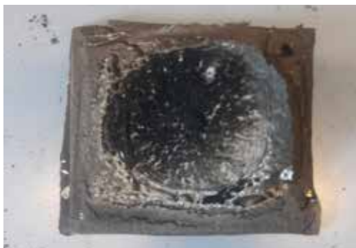
Figure 18: Al-sheet coated with EP-resin with 300 phr ACTILOX® HTB after torch flame test. Left: exposed (coated) side showing ceramic like residue, right: backside showing intact Al.
