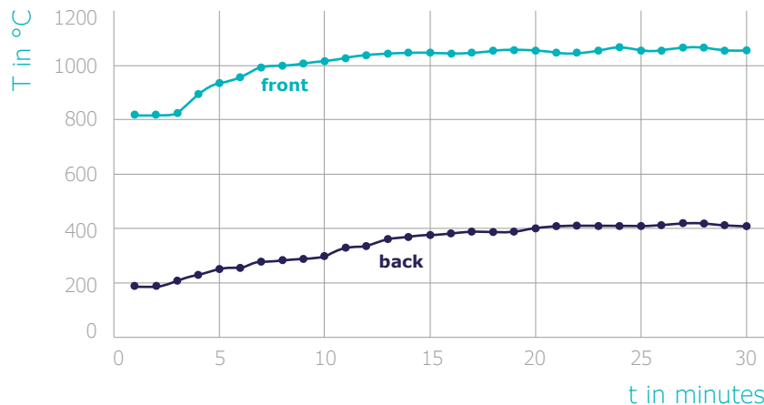
Figure 22: Temperature recording over 30 min torch-test on ACTILOX® HTB containing laminate B) for front side (light blue, exposed to flame) and back side (dark blue).
