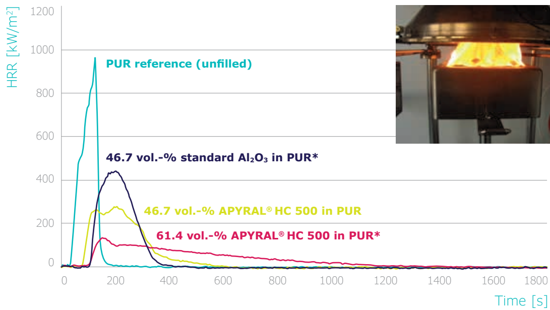
Figure 16: Cone measurement of PUR. Heat release rate of unfilled PUR in comparison with APYRAL® HC 500 and standard Al 2 O 3 filled PUR (*max. Possible filling level in this resin based on Caradol(R) 34-08, Shell).
