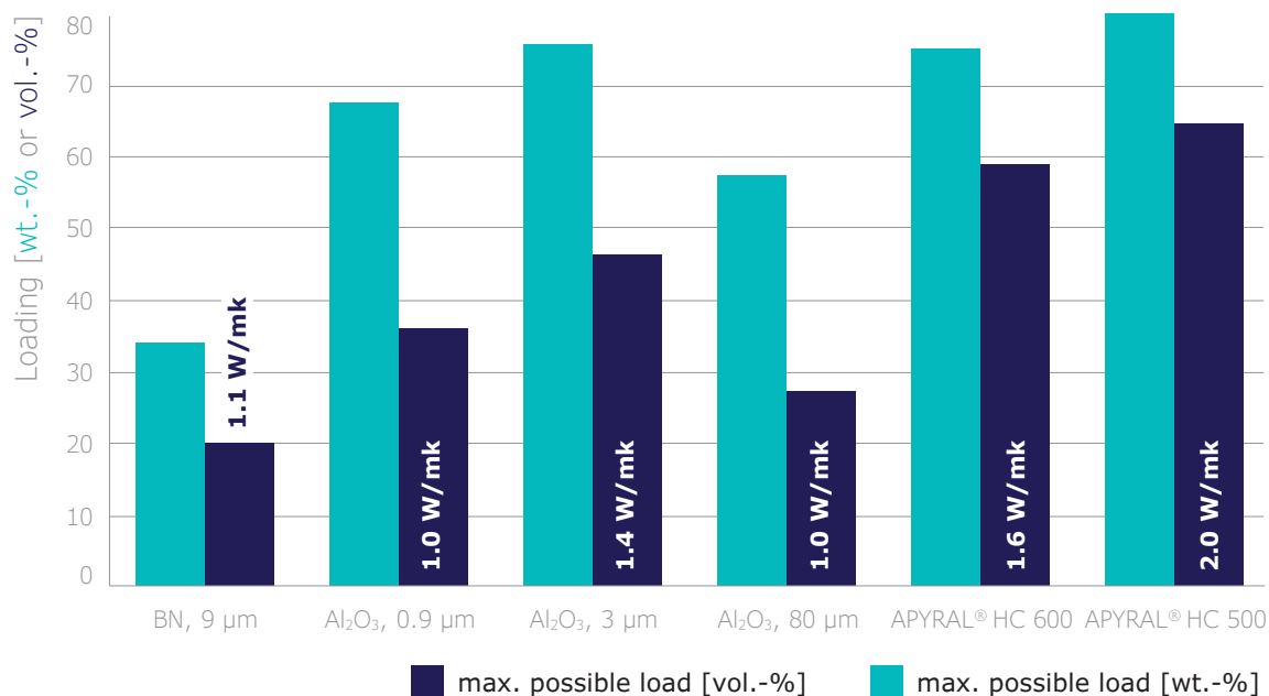
Figure 13: TC of APYRAL® HC in comparison to calcined alumina, and BN in UP-resin at 22 °C (Hot Disk method).
