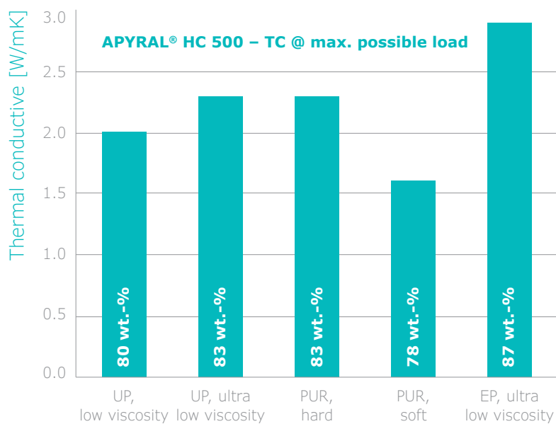
Figure 14: Thermal conductivity of selected resins of various chemistry and cross linking density filled with APYRAL® 500 HC to the maximum possible load in each resin.
