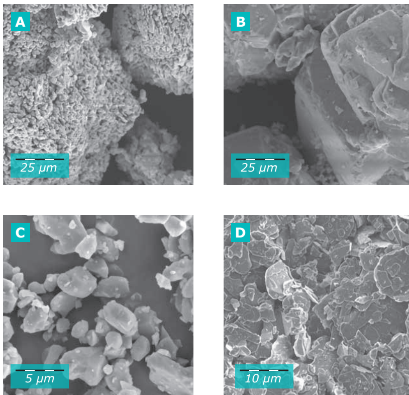
Figure 10: SEM-images of calcined alumina (80 µm, A), APYRAL® HC 500 (B), calcined alumina (3 µm, C), and BN (9 µm, D).
