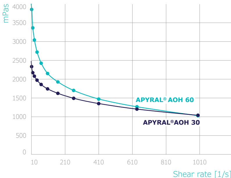
Figure 5: Viscosity as a function of shear rate for electrode-coating slurries. Influence of the fineness of the used boehmite ( APYRAL® AOH 30 vs. APYRAL® AOH 60 ) is demonstrated using a solid content of 40 %.
