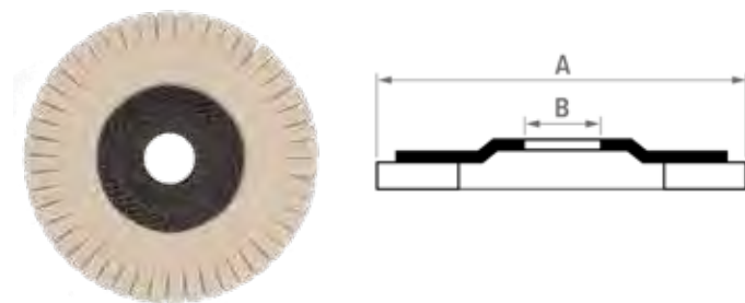
Type FG 27 (flat) reduced backing
